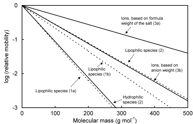
FIG. 2. Correlations between the molecular mass of lipophilic (dashed lines) and hydrophilic solutes (solid lines) and their relative mobility across atomatous isolated cuticles of different plant species. Based on data from: (1) Buchholz et al. (1998) ( Populus alba ), (2) Popp et al. (2005) ( Hedera helix ) (3): Schönherr and Schreiber (2004) ( Populus canescens ). For comparability, the mobility of a molecule with zero molecular weight was set to zero. Data from (1) were converted into molecular mass using: (1a) the conversion proposed by (3) or (1b) linear regression calculated from data given in (2). Data from (3) are presented as given by the authors (3a) and recalculated (3b) to show the dependence of mobility on the weight of the largest ion instead of the gross formula mass of the salt.
