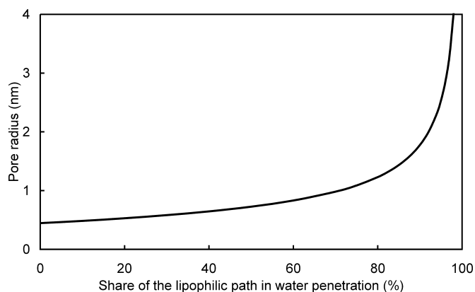
FIG. 3. Dependence of values of pore radii on the actual share of water penetration across the lipophilic route across cuticles of C. aurantium . Data were taken from Table 9 and pore radii were calculated with Equation 13 given in Schönherr (1976a), assuming that the diffusional flow of water is composed of flow across both the lipophilic and the hydrophilic path. The radius of 0.45 nm at 0% share is the value reported by Schönherr (1976a).
