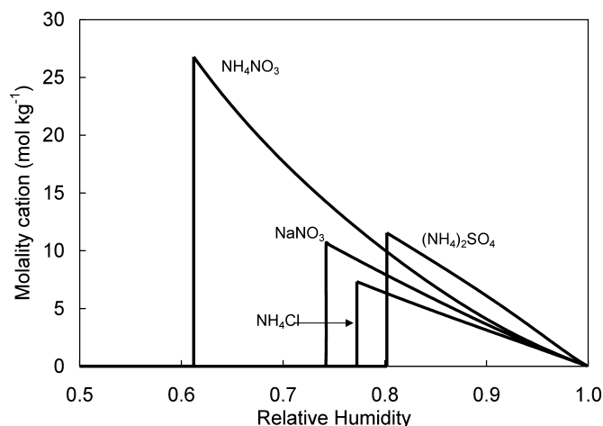
FIG. 4. Equilibrium concentrations of some N-salt aerosols as effected by relative ambient air humidity. At the respective DRH of a salt a sudden transition between the solid and the dissolved state occurs. Data were calculated using the Extended Aerosol Inorganics Model of Clegg, Brimblecombe and Wexler ( http://www.aim.env.uea.ac.uk/aim/aim.php ) for a cation concentration of 1 \text{ mol m}^{-3} air.
