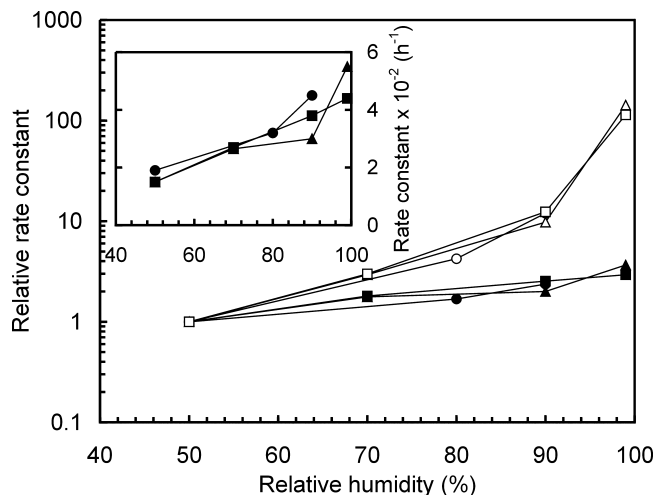
FIG. 5. Rate constants of diffusion of \text{Ca}^{2+} and \text{Rb}^{+} across isolated astomatous pear cuticles as affected by relative air humidity. Note the logarithmic scale of the ordinate. Recalculated data from: Schönherr (2000), \text{Ca}^{2+} , triangles; Schönherr (2001), \text{Ca}^{2+} , squares; Schönherr and Lubert (2001), \text{Rb}^{+} , circles. Values are expressed relative to the rate constant measured at 50% RH, which was set to 1. Filled symbols are based on the original data presented by the authors. Open symbols are recalculated values obtained by dividing the rate constants by the equilibrium concentration of the salt at the respective humidity. Equilibrium concentrations were calculated using tabulated solubility data assuming maximum concentrations at the deliquescence humidity of each salt, a linear decrease of concentration with increasing humidity, and a concentration of zero at 100% humidity. The insert shows the absolute values of rate constants as given by the authors.
